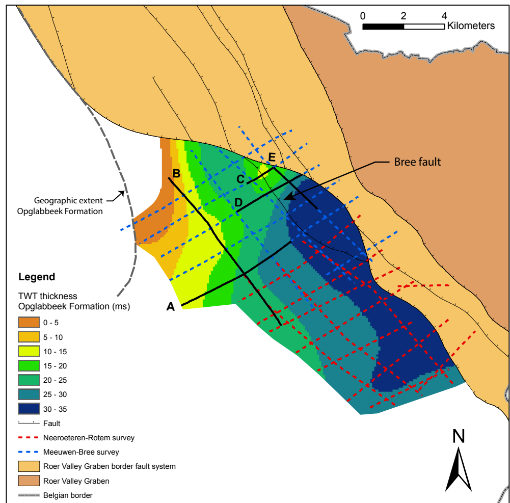
Figure 7. Schematic two-way-travel time thickness (isochronopach) map of the Opglabbeek Formation in the study area.
