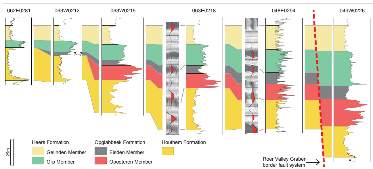
Figure 5. Well log and seismic interpretations from the Roer Valley Graben in the east towards the SECB in the west. The well log interpretations are extracted from De Koninck et al. (2011) and are presented on top of the gamma-ray logs. The black lines connect the well log interpretations to the corresponding red wiggles of the synthetic seismogram that are displayed on part of a reflection seismic line. The location of this trace is given in figure 3.
