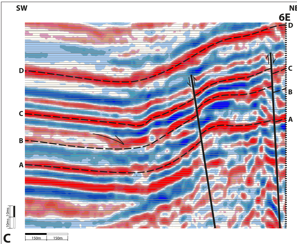
Figure 6. Seismic sections across the study area. Locations are given in figure 2. A. SW-NE section that shows the south-west directed thinning of the Opglabbeek and Heers Formations in the north-western sector. The top of the Heers Formation is flattened. B. NW-SE section that shows the north-west directed thinning of the Opglabbeek and Heers Formations in the north-western sector. The top of the Heers Formation is flattened. See figure 6A for the legend. C & D. SW-NE sections across the northern part of the Bree Uplift. These sections show that the Opglabbeek Formation thins on top of the forced folded Bree Uplift and that the Heers Formation thins only on fault blocks that pop-up in between oppositely dipping reverse faults. See figure 6A for the legend. E. NW-SE section along the northern part of the Bree Uplift and along the footwall to the north-easternmost fault of figure 6C. The Opglabbeek Formation thins towards the north-west as the northern part of the Bree Uplift was folded into an anticline during the latest Danian. The thickness of the Heers Formation hardly changes along this section since the hangingwall block and not the footwall block to the north-easternmost fault of figure 6C was uplifted. The top of the Heers Formation is flattened. See figure 6A for the legend
