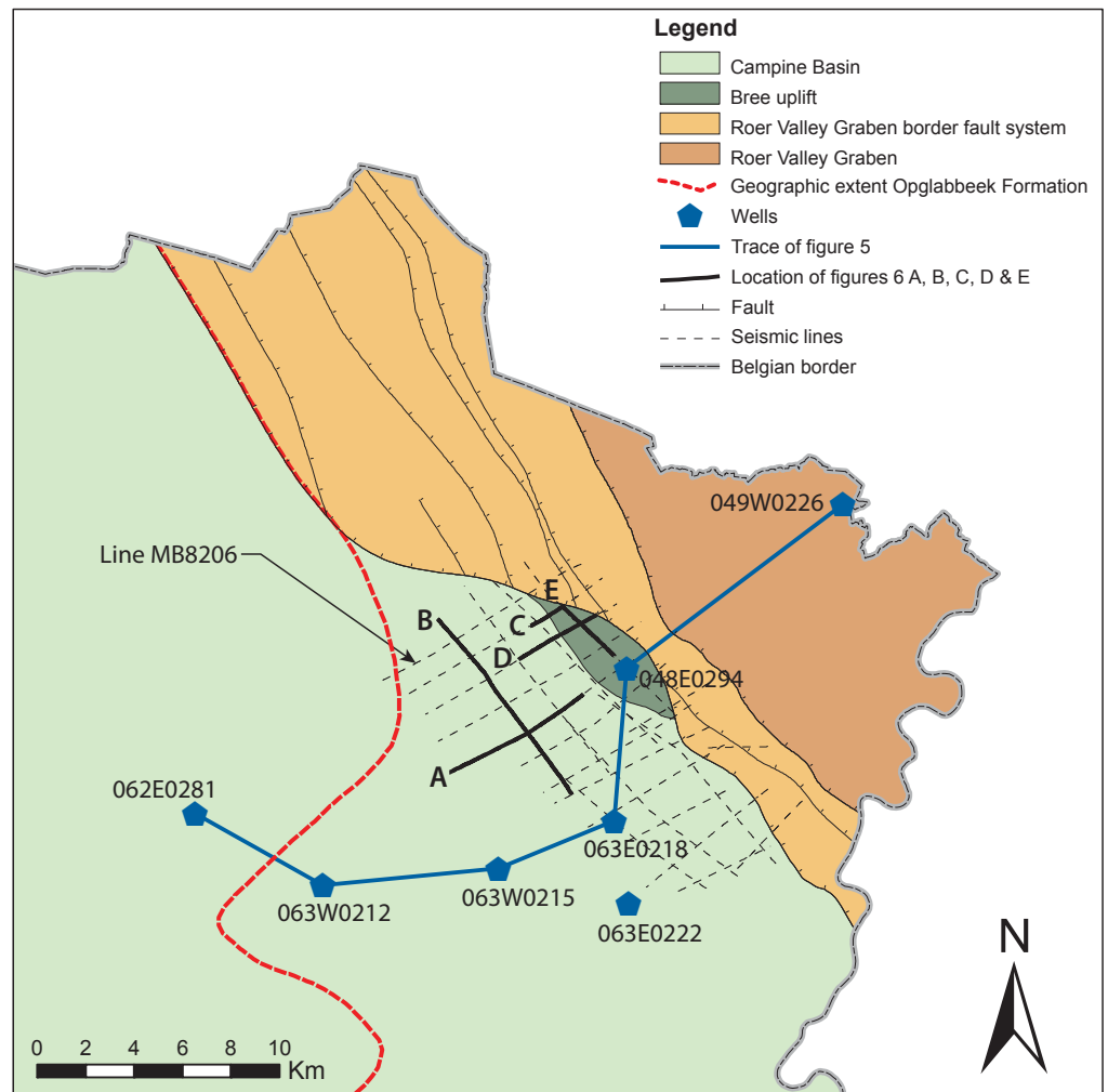
Figure 3. Overview of the south-eastern part of the Campine Basin and the Belgian sector of the Roer Valley Graben. The geographic extent of the Opglabbeek Formation was modified after the G3Dv2-model (Matthijs et al., 2013).
