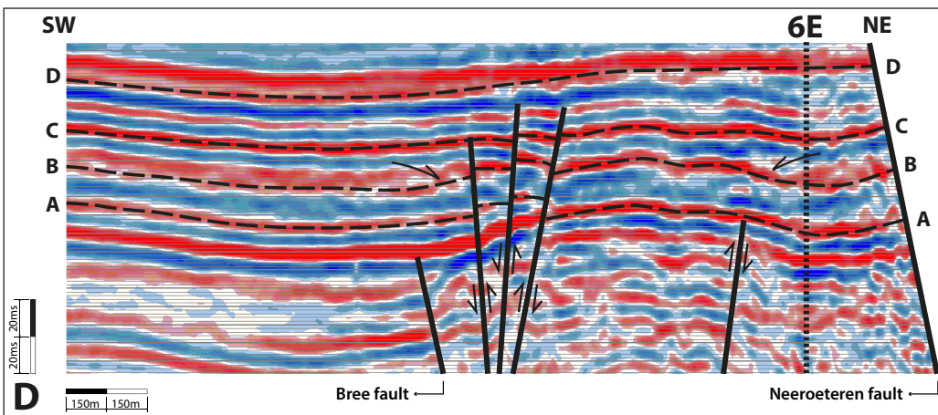
Figure 6. Seismic sections across the study area. Locations are given in figure 2. A. SW-NE section that shows the south-west directed thinning of the Opglabbeek and Heers Formations in the north-western sector. The top of the Heers Formation is flattened. B. NW-SE section that shows the north-west directed thinning of the Opglabbeek and Heers Formations in the north-western sector. The top of the Heers Formation is flattened. See figure 6A for the legend. C & D. SW-NE sections across the northern part of the Bree Uplift. These sections show that the Opglabbeek Formation thins on top of the forced folded Bree Uplift and that the Heers Formation thins only on fault blocks that pop-up in between oppositely dipping reverse faults. See figure 6A for the legend. E. NW-SE section along the northern part of the Bree Uplift and along the footwall to the north-easternmost fault of figure 6C. The Opglabbeek Formation thins towards the north-west as the northern part of the Bree Uplift was folded into an anticline during the latest Danian. The thickness of the Heers Formation hardly changes along this section since the hangingwall block and not the footwall block to the north-easternmost fault of figure 6C was uplifted. The top of the Heers Formation is flattened. See figure 6A for the legend
