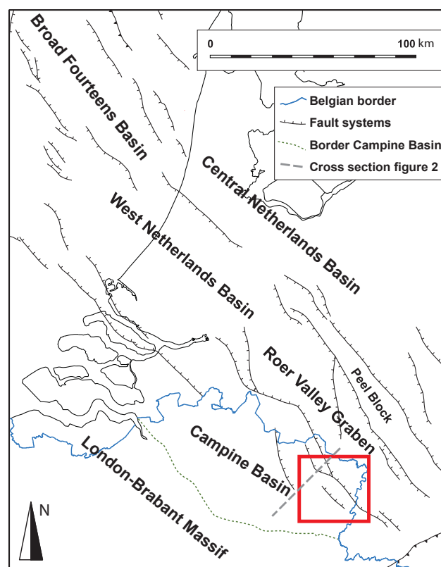
Figure 1. Structural elements map of the Netherlands and northern Belgium showing the Jurassic and Early-Cretaceous basins, highs and platforms (modified after De Jager, 2007). The study area is indicated by the red rectangle.
